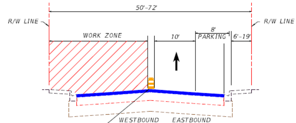
CHANNELIZING DEVICE PHASE II 13TH STREET TO SR-5/US-1 WESTBOUND DETOUR
