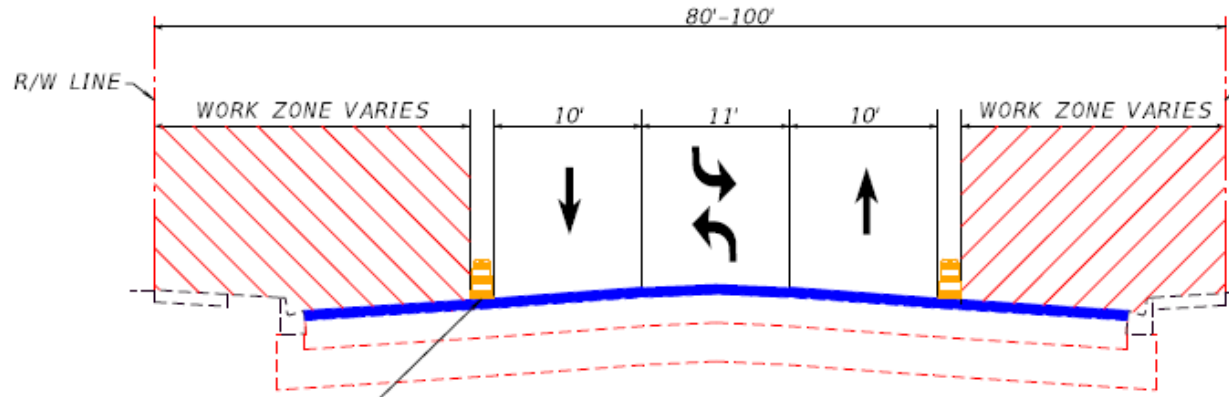
CHANNELIZING DEVICE PHASE I 32ND STREET TO 13TH STREET
