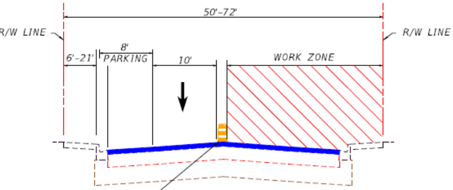
CHANNELIZING DEVICE PHASE I 13TH STREET TO SR-5/US-1 EASTBOUND DETOUR
