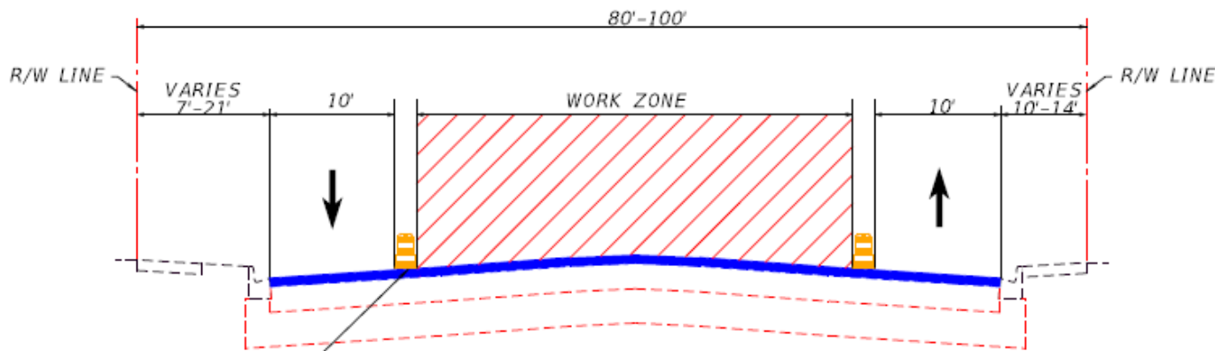
CHANNELIZING DEVICE PHASE II 32ND STREET TO 13TH STREET
